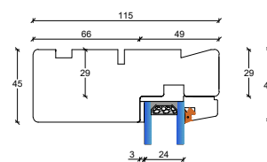
D6: Faste elementer, top karm
